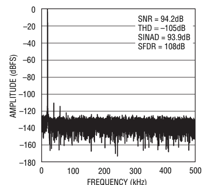
16k Point FFT f_s = 1\text{Mps} , f_{\text{IN}} = 20\text{kHz}
