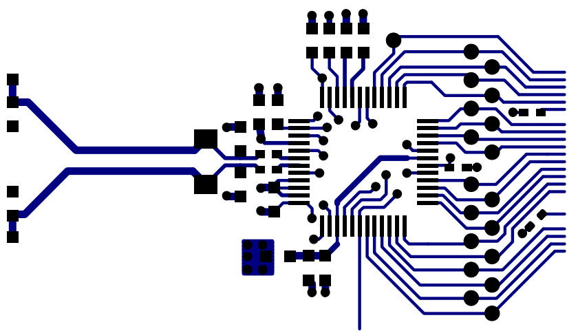
Partial Layer 1 Component Side
