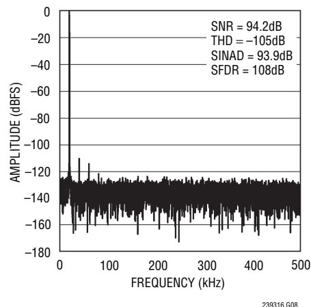
Figure 5. 16k Point FFT of the LTC2393-16, f_s = 1\text{Msps} , f_{IN} = 20\text{kHz}
